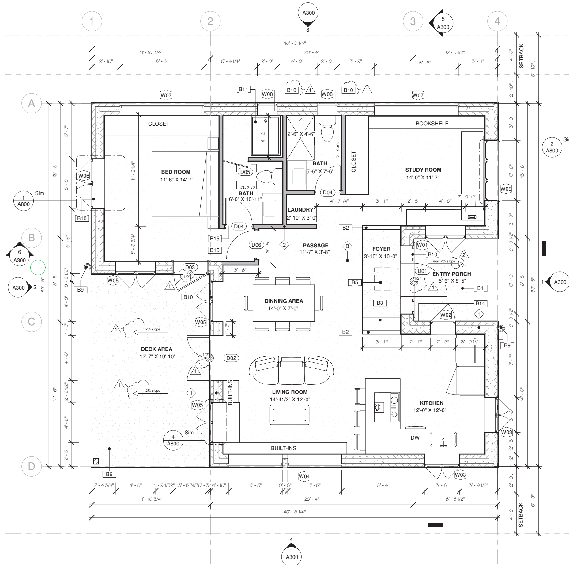
1 PROPOSED PLAN- GROUND LEVEL 1,175 SF SCALE 1/4" = 1'-0"
